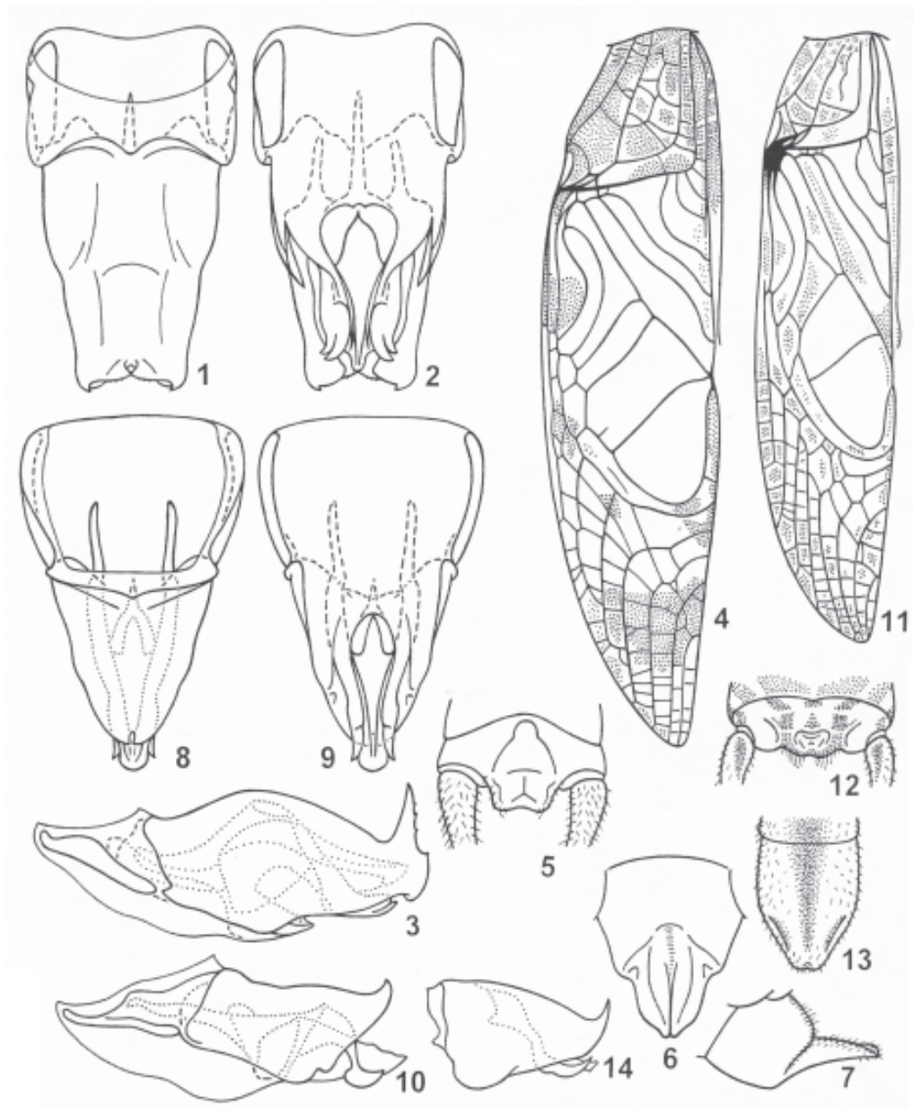
Figs VIII (1-14). Varitrella , male. 1-7 , V. nigrifrons (Chop.) (holotype); 8-13 , V. varipennis (Walk.) (holotype); 14 , V. sp. (from Chopard, 1936: Fig. 20). Genitalia from above (1, 8), from below (2, 9), and from side (3, 10); dorsal part of tegmen (4, 11); anal (5, 12) and genital (6, 7, 13) plates from above and slightly from behind (5, 12), from below (6, 13), and from side (7); distal part of genitalia from side (14).
