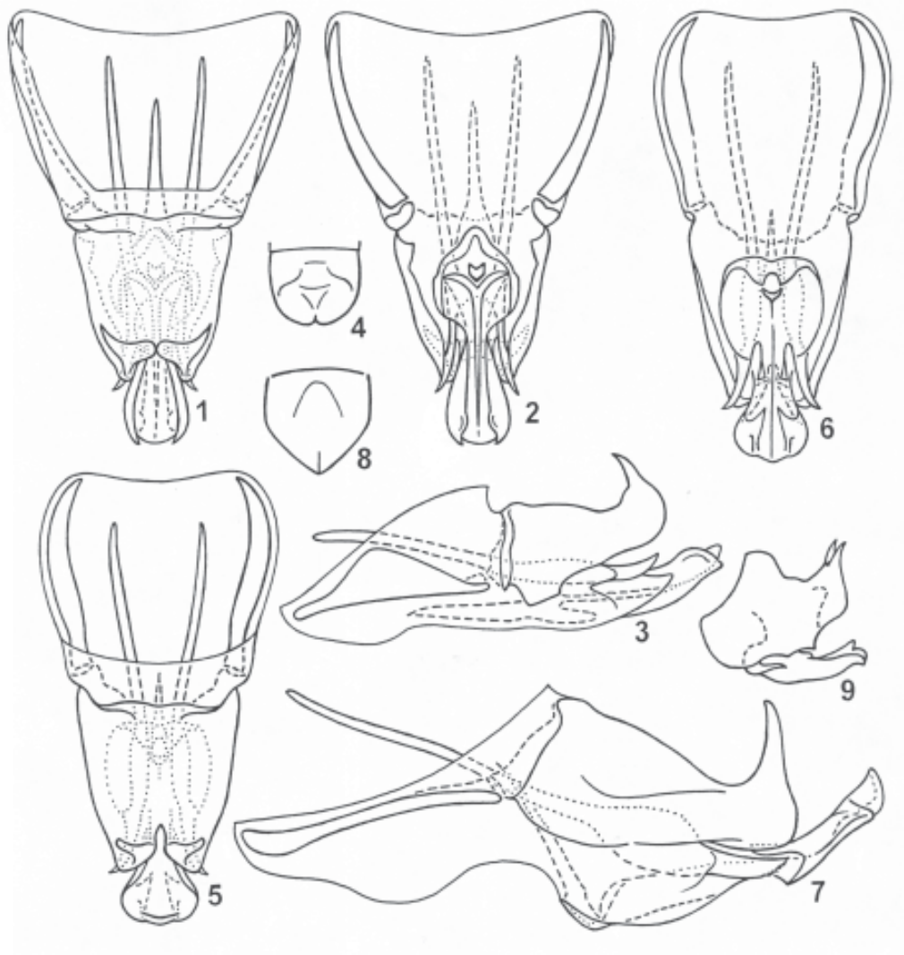
Figs XI (1-9). Mnesibulus , male. 1-4 , M. pallidulus Bol. (lectotype); 5-8 , M. malacca sp. n.; 9 , M. striatipes Chop. (from Chopard, 1969). Genitalia (1-3, 5-7) and their distal half (9) from above (1, 5), from below (2, 6), and from side (3, 7, 9); genital plate from below (4, 8).
