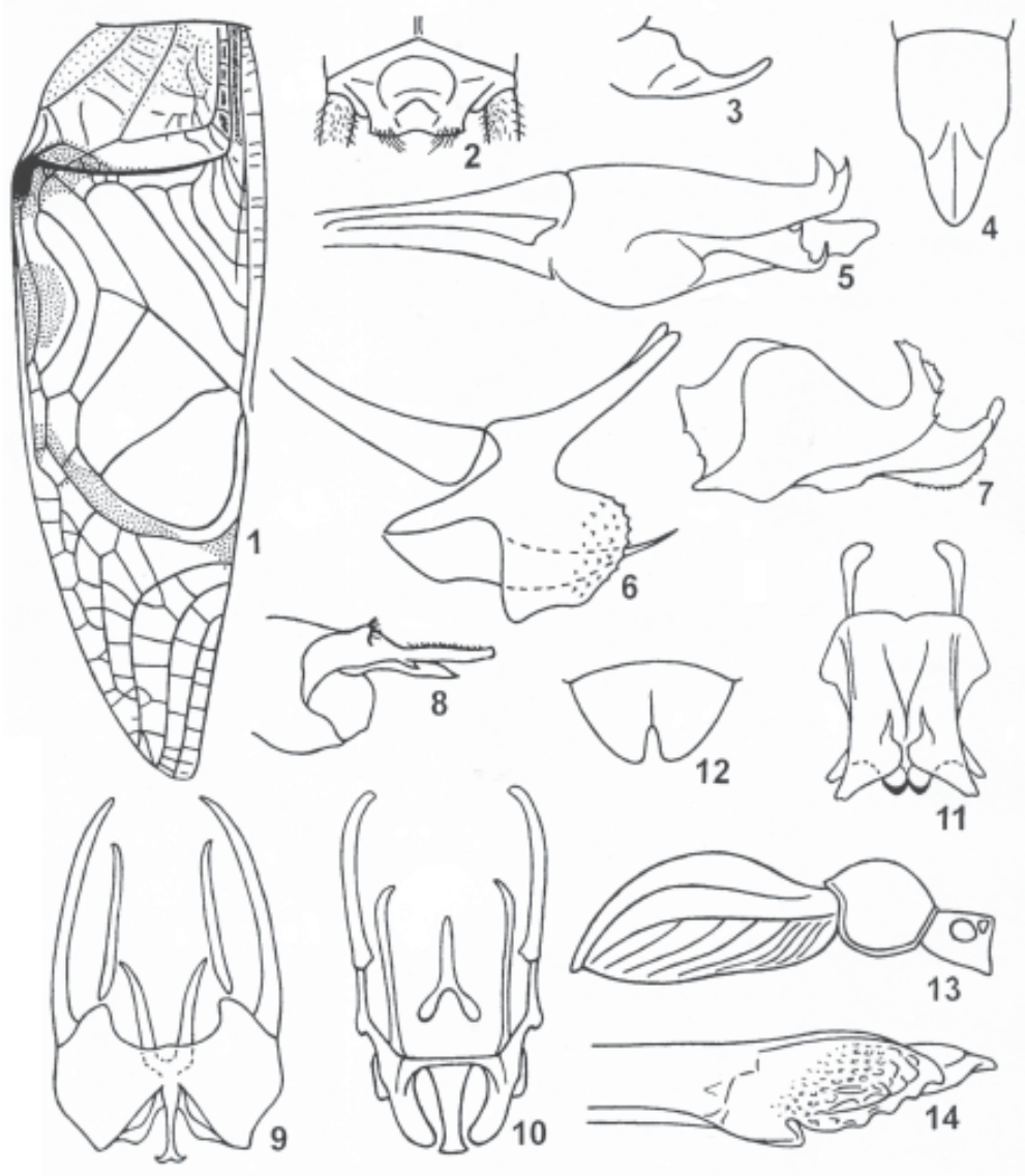
Figs XIV (1-14). Indisputable and possible Podoscirtini. 1-5 , Madasumma? fletcheri Chop. (holotype; 5, from Chopard, 1935); 6 , M.? valida Chop. (from Chopard, 1936); 7 , M.? melanotum Chop. (from Chopard, 1969); 8 , Mnesibulus? andrewesi Chop. (from Chopard, 1928); 9 , M.? pallipes Chop. (from Chopard, 1936); 10 , Corixogryllus abbreviatus Bol. (from Chopard, 1969); 11 , Aphonoides? griseipennis Chop. (from Chopard, 1969); 12-14 , Scepastus pachyrrhynchoides Gerst. Dorsal part of male tegmen (1); anal (2) and genital (3, 4, 12) plates of male (2-4) and female (12) from above (2), from side (3), and from below (4, 12); male genitalia from side (5-8) and from above (9-11); general appearance of head, pronotum, and tegmina from side (13); apex of ovipositor from side (14).
