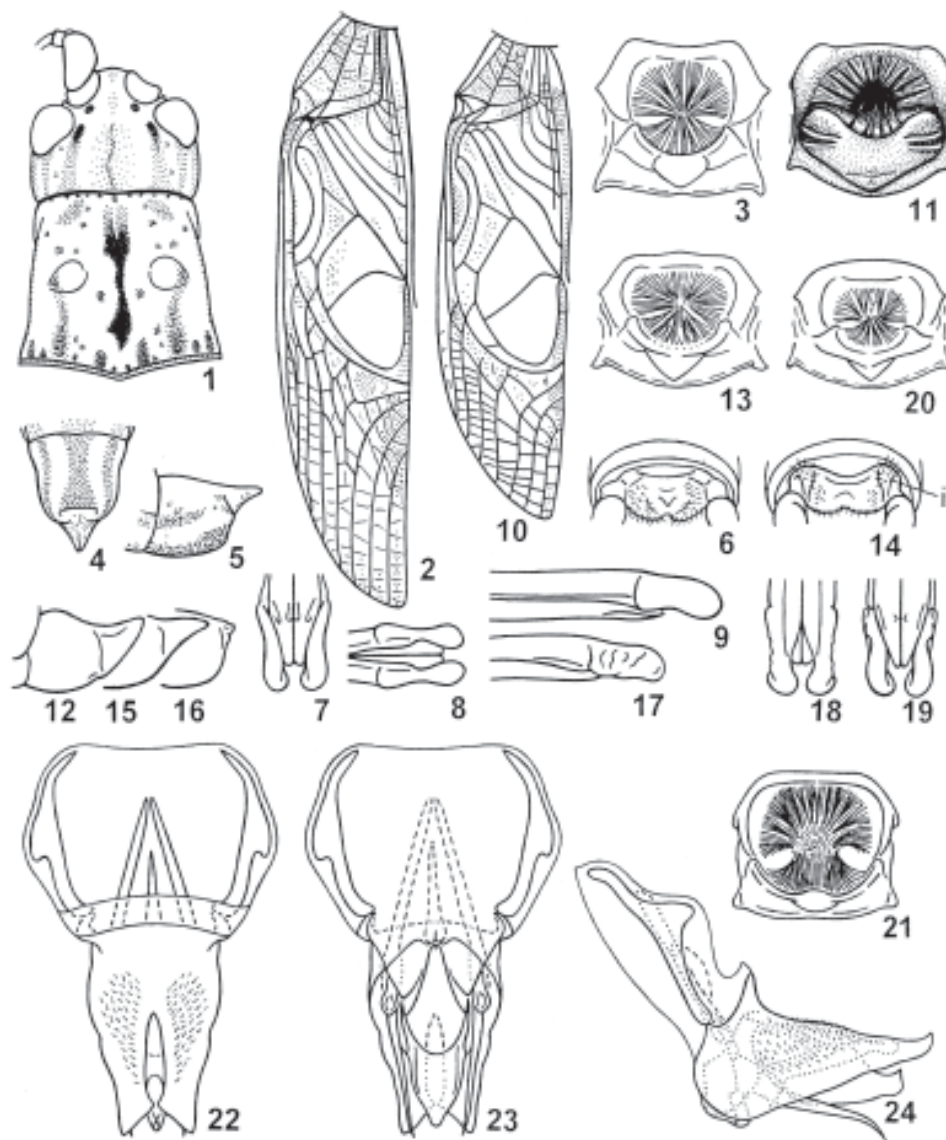
Figs I (1-24). Noctitrella . 1-9 , N. spinosa sp. n.; 10-12 , N. tranquilla Gor. (holotype); 13-19 , N. ardua sp. n. (13, 14, 16, holotype); 20 , N. parardua sp. n.; 21-24 , N. berezini sp. n. Head of male with pronotum (1), dorsal part of male tegmen (2, 10), and male metanotal gland (3, 11, 13, 20, 21) from above; anal (6, 14) and genital (4, 5, 12, 15, 16) plates of male from behind and slightly from above (6, 14), from below (4), and from side (5, 12, 15, 16); apex of ovipositor from below (7, 19), from above (8, 18), and from side (9, 17); male genitalia from above (22), from below (23), and from side (24). Abbreviation: i, inflation with hairs.
