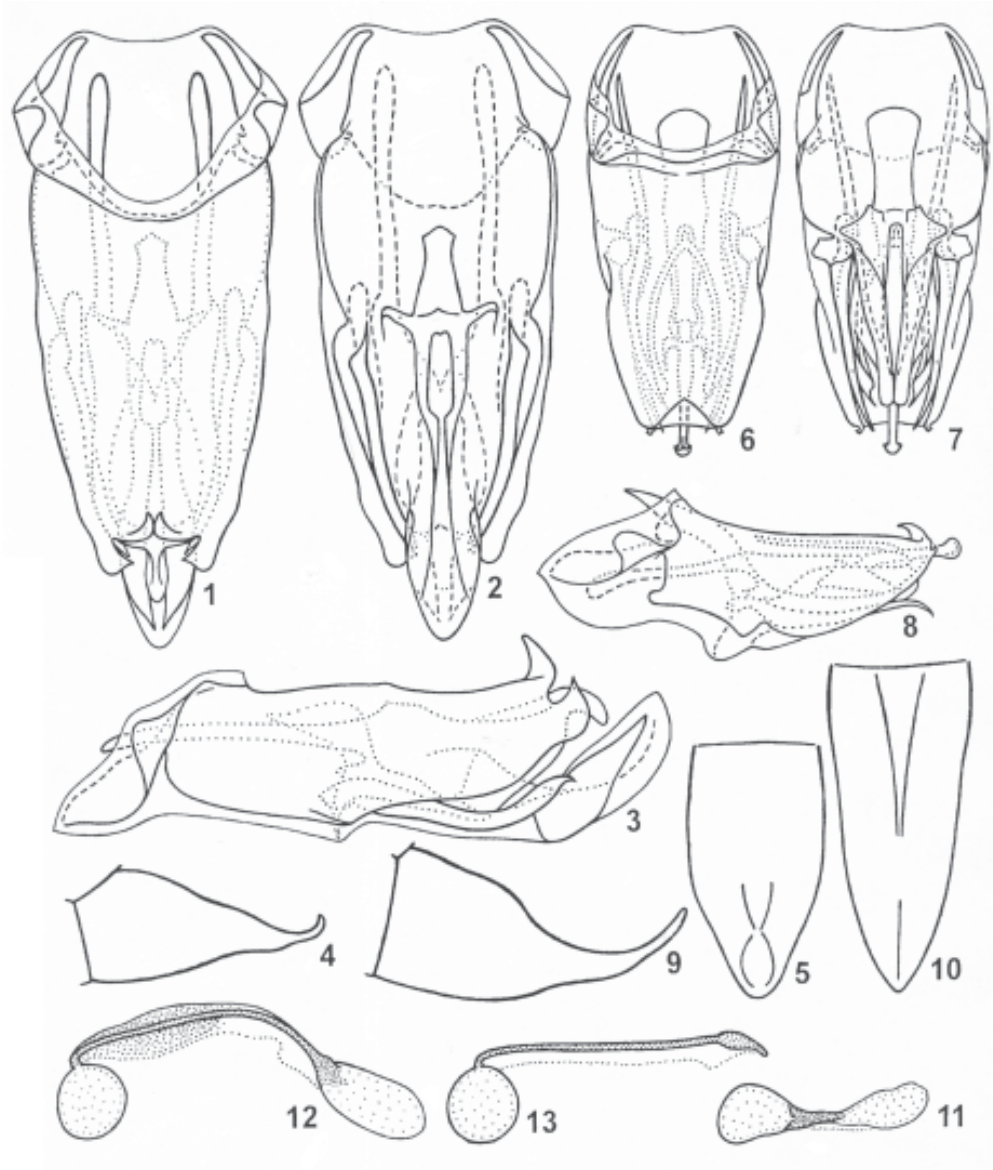
Figs XVII (1-13). Hemitrella , male. 1-5 , H. halmaherae sp. n.; 6-11 , H. cyclopea sp. n. (holotype); 12 , H. proxima sp. n.; 13 , H. papuana sp. n. (holotype). Genitalia from above (1, 6), from below (2, 7), and from side (3, 8); genital plate from side (4, 9) and from below (5, 10); spermatophore from side (11-13).
