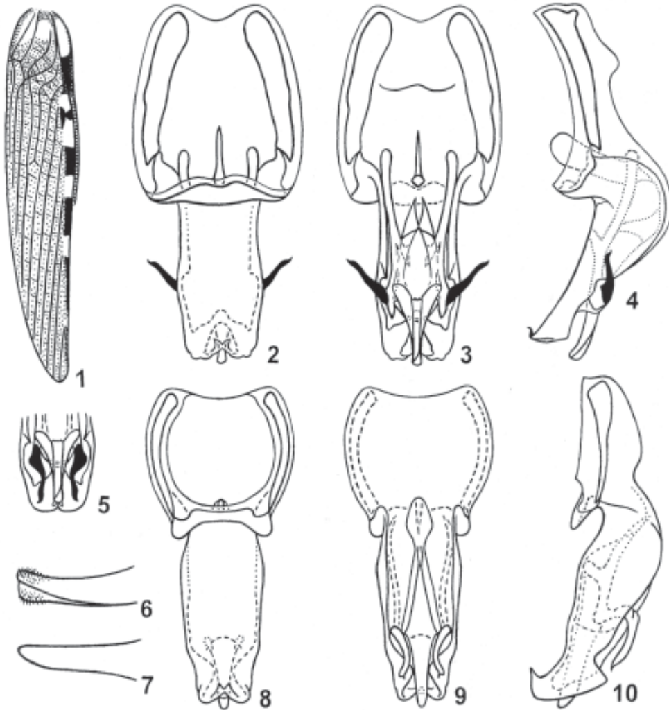
Figs XIX (1-10). Matuanus , male. 1-6 , M. priapus (Sauss.) (neotype); 7-10 , M. rufomaculatus sp. n. Dorsal part of tegmen (1); genitalia from above (2, 8), from below (3, 9), and from side (4, 10); distal part of genitalia with other position of ectoparameres from below (5); guiding rod from side (6, 7).
