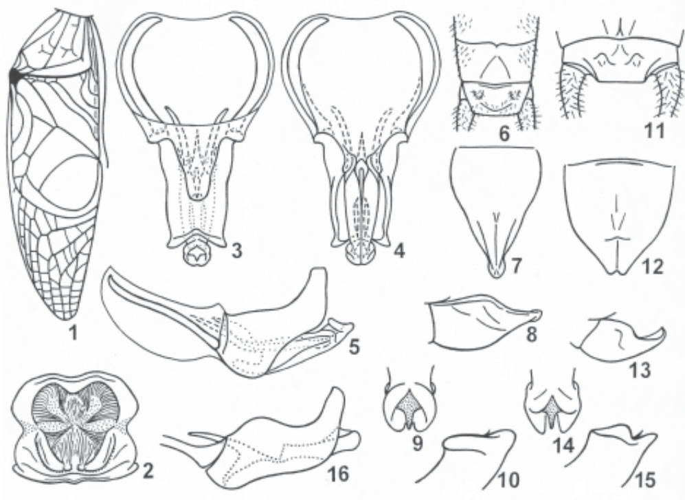
Figs V (1-16). Poliotrella , male. 1-10 , P. zaitzevi Gor. (holotype); 11-15 , P. greeni (Chop.) (lectotype); 16 , P.? albonotata (Chop.) (from Chopard, 1936). Dorsal part of tegmen (1); metanotal gland from above (2); genitalia from above (3), from below (4), and from side (5, 16); distal part of abdomen from above (6, 11); genital plate from below (7, 12) and from side (8, 13); apex of guiding rod from above (9, 14) and from side (10, 15).
