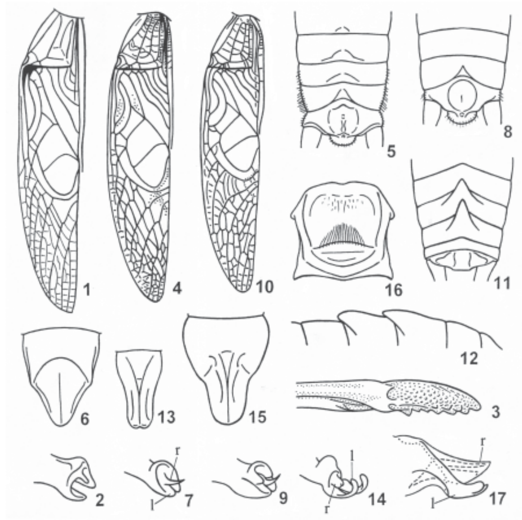
Figs VI (1-17). Varitrella . 1-3, V. quadrata (Haan); 4-7, V. conspersa (Stål) (holotype); 8, 9, V. depressa sp. n.; 10-14, V. saussurei (Stål) (holotype); 15, V. ?bakeri (Chop.); 16, 17, V. nigrifrons (Chop.). Dorsal part of male tegmen (1, 4, 10); apex of guiding rod from side and slightly from below (2, 7, 9, 14); apex of ovipositor from side (3); distal part of male abdomen from above (5, 8, 11) and upper part of its tergites from side (12); male genital plate from below (6, 13, 15); metanotal gland from above (16); guiding rod from side (17). Abbreviations: l , lateral lobe; r , inner rod.
