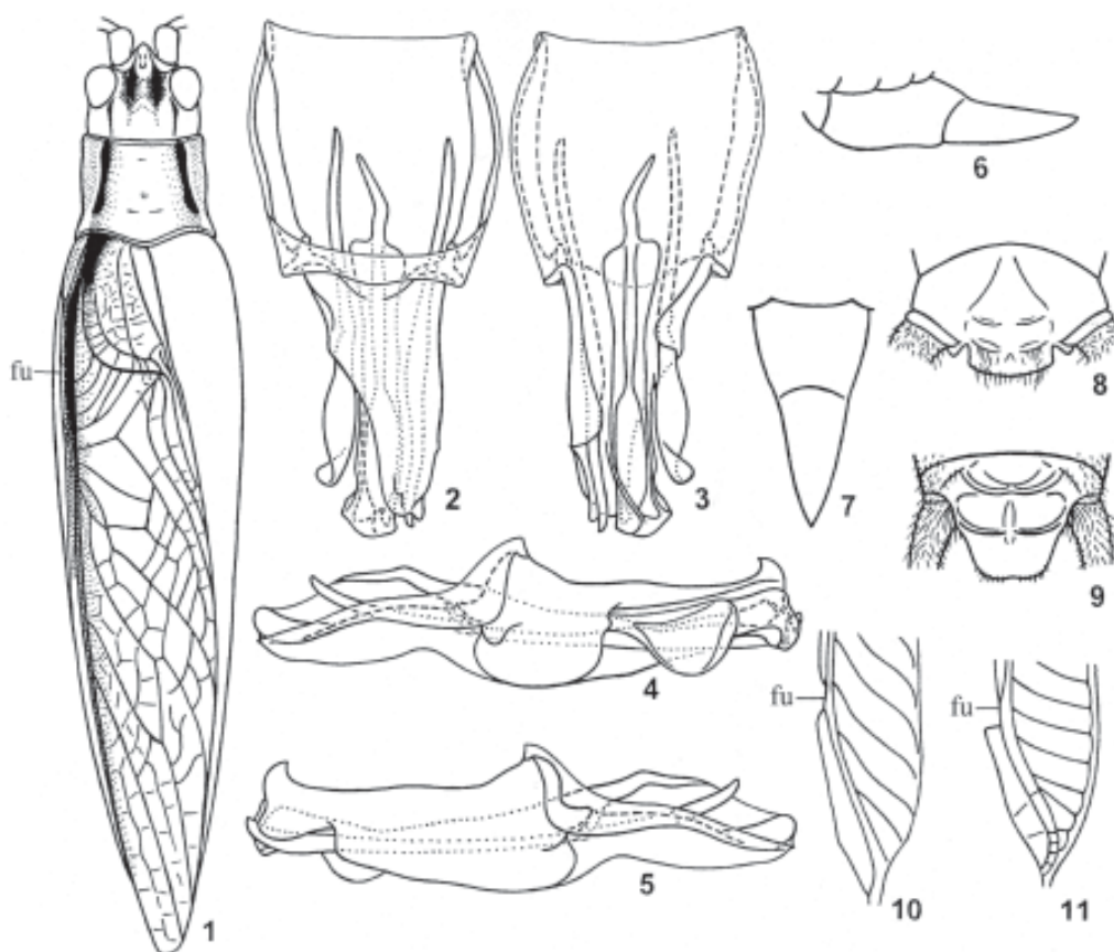
Figs XX (1-11). Hemiphonus , Matuanus and Tamborina , male. 1-8 , H. wilparina Otte & Alex.; 9 , M. rufomaculatus sp. n.; 10 , T. australis (Walk.); 11 , T. ? affinis (Chop.). Head, pronotum and left tegmen from above (1); genitalia from above (2), from below (3), and from side (4, 5); genital (6, 7) and anal (8, 9) plates from side (6), from below (7), and from above (8, 9); distal half of lateral part of tegmen (10, 11) (from Otte & Alexander, 1983). Abbreviation: fu, fusion of R with M .
