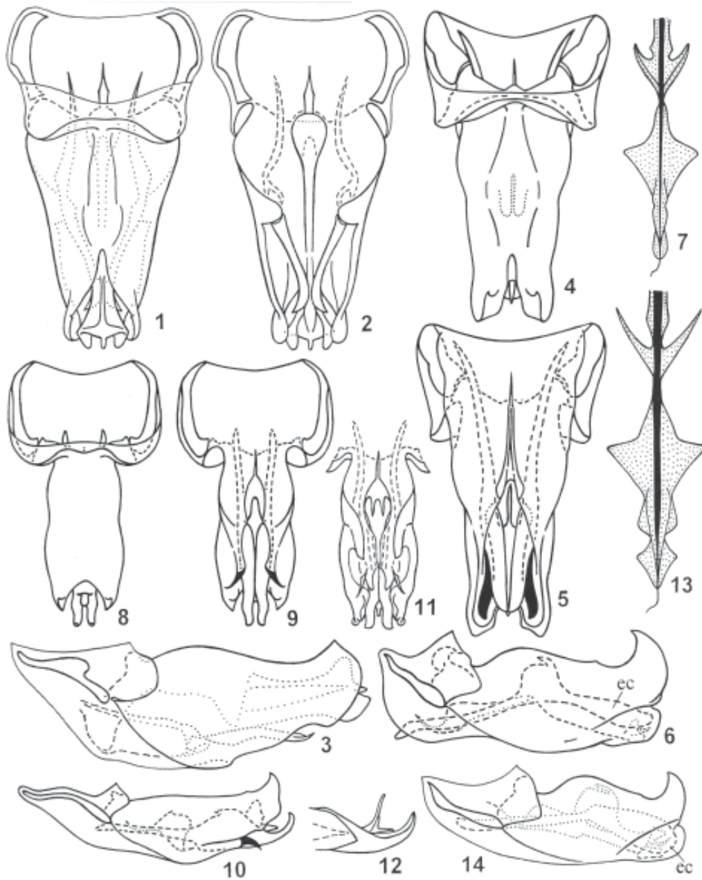
Figs VII (1-14). Varitrella , male. 1-3 , V. quadrata (Haan); 4-7 , V. conspersa (Stål) (holotype); 8-10 , V. saussurei (Stål) (holotype); 11, 12 , V. ?bakeri (Chop.); 13, 14 , V. depressa sp. n. Genitalia from above (1, 4, 8), from below (2, 5, 9, 11; in Fig. 11 rami not shown), and from side (3, 6, 10, 14); attachment plate of spermatophore from below (7, 13); guiding rod from side (12). Abbreviation: ec , inner sclerotised part of ectoparamere.
